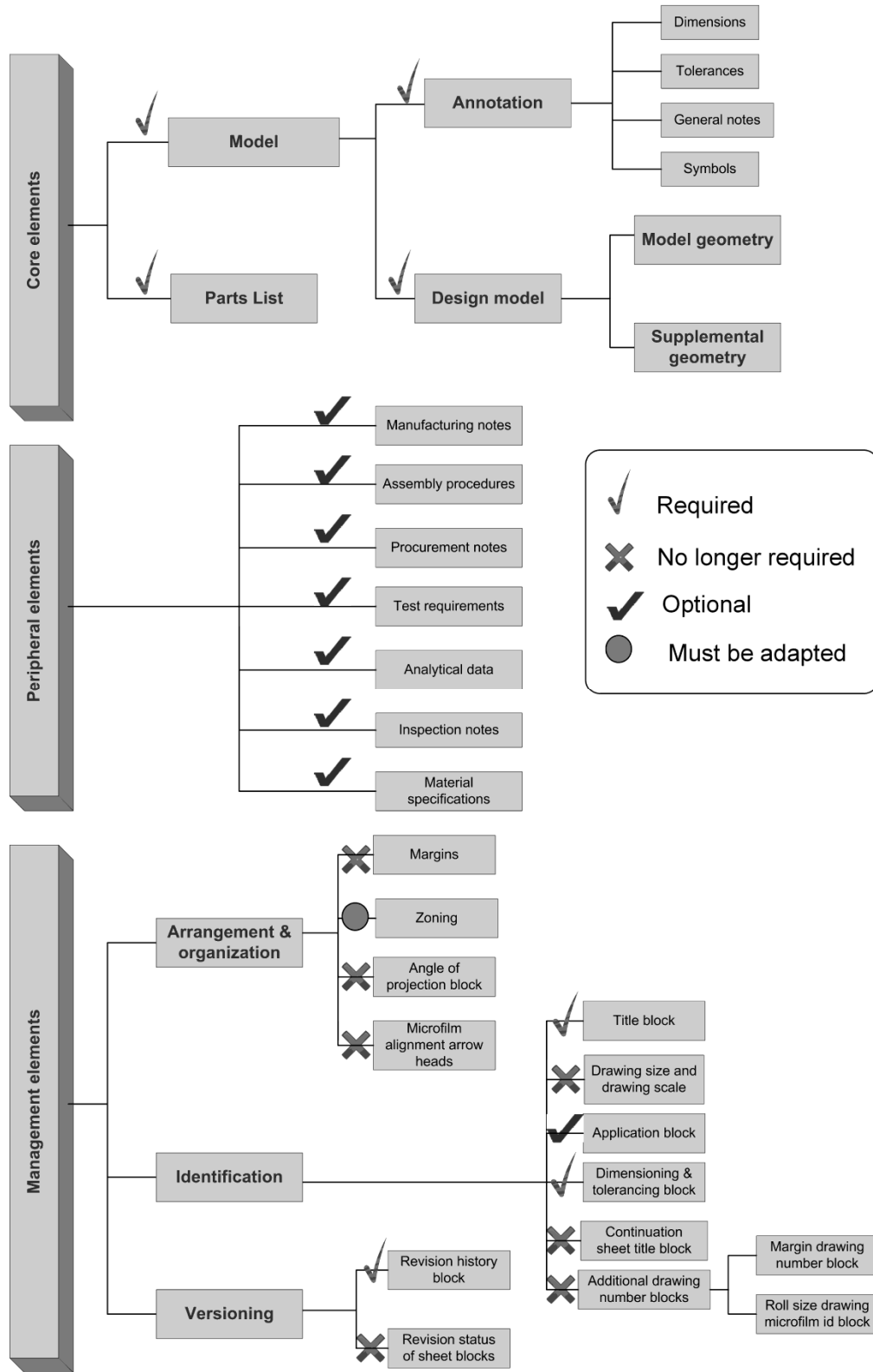
Figure 3 – Drawing elements: classification and transfer to MBD
